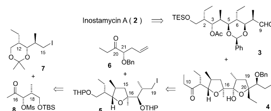
Scheme 1. Retrosynthetic analysis.
