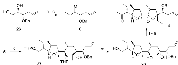
Scheme 4. Reagents and conditions. a) \text{NaIO}_4 , \text{H}_2\text{O} , THF, 0^\circ\text{C} ; b) \text{EtMgBr} , THF, -78^\circ\text{C} ; c) DMP, \text{CH}_2\text{Cl}_2 , 25^\circ\text{C} , 71% (over 3 steps); d) t\text{BuLi} , THF, -78^\circ\text{C} , then \text{LaCl}_3 \cdot 2\text{LiCl} in THF, -78^\circ\text{C} , then 6 in THF, -78^\circ\text{C} ; e) PPTS, EtOH, 40^\circ\text{C} , 79% (over 2 steps); f) TEMPO, \text{PhI}(\text{OAc})_2 , \text{CH}_2\text{Cl}_2 , 0 to 25^\circ\text{C} ; g) \text{EtMgBr} , THF, -78^\circ\text{C} ; h) AZADO, \text{PhI}(\text{OAc})_2 , \text{CH}_2\text{Cl}_2 , 0 to 25^\circ\text{C} , 81% (over 3 steps). DMP = Dess–Martin periodinane, TEMPO = 2,2,6,6-tetramethylpiperidine 1-oxyl, AZADO = 2-azaadamantane N -oxyl.
