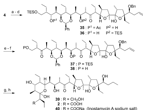
Scheme 6. Reagents and conditions. a) \text{TMP-HBr} , n\text{BuLi} , THF, -78^\circ\text{C} , then 3 in THF, -78^\circ\text{C} , 92%; b) TESOTf, 2,6-lutidine, \text{CH}_2\text{Cl}_2 , -78^\circ\text{C} , 94%; c) PPTS, EtOH, -20^\circ\text{C} , then \text{K}_2\text{CO}_3 , -20 to 25^\circ\text{C} ; d) \text{TESCl} , \text{Et}_3\text{N} , \text{CH}_2\text{Cl}_2 , -78^\circ\text{C} , 94% (over 2 steps); e) AZADO, \text{PhI}(\text{OAc})_2 , \text{CH}_2\text{Cl}_2 , Py, 0 to 25^\circ\text{C} , 92%; f) \text{Et}_3\text{N} \cdot 3\text{HF} , MeCN, 25^\circ\text{C} , 92%; g) \text{H}_2 , 10% Pd/C, Amberlite IRA-67, EtOH, 25^\circ\text{C} , 94%; h) TEMPO, \text{NaOCl} , pH 6.7 phosphate buffer, \text{H}_2\text{O} , MeCN, 25^\circ\text{C} , then aq \text{Na}_2\text{S}_2\text{O}_3 , aq \text{NaHCO}_3 , 84%.
